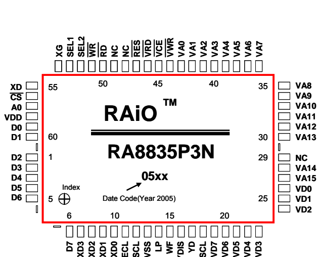
Figure 4-1: RA8835P3N(QFP-60 Pin)
