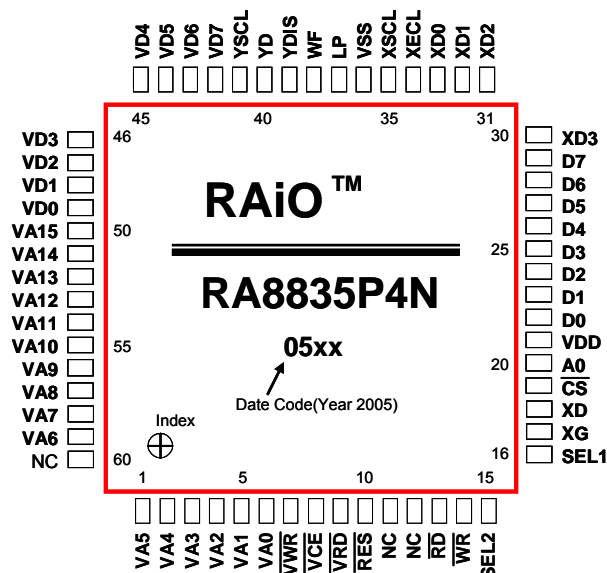
Figure 4-2: RA8835P4N (TQFP-60 Pin)
